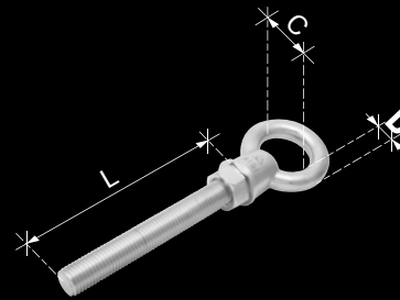
M J S307 Metric Imperial Lifting eye bolt (with washer and nut)
