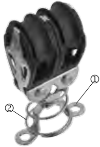
Double stand-up (incl. ① 2-P eye 403-122, ② stand-up spring 403-123)
